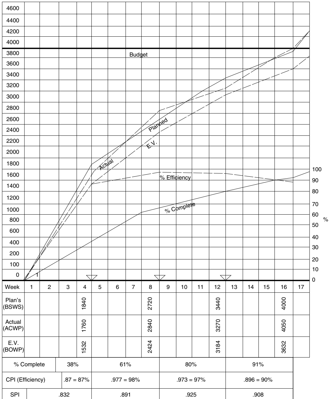
Figure 48.13 Control curves
