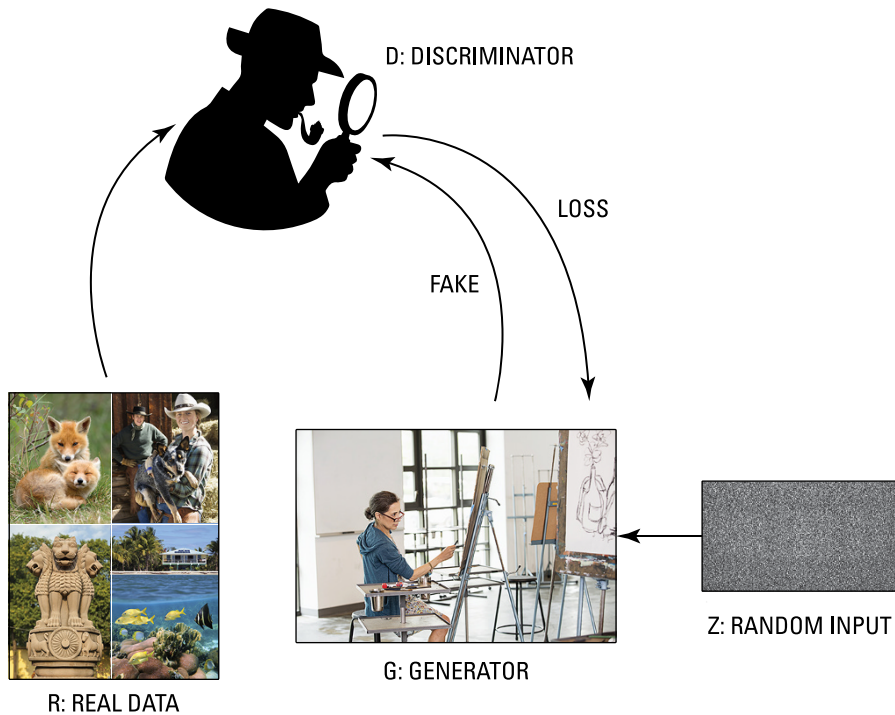
FIGURE 11-5: How a GAN network works, oscillating between generator and discriminator.
