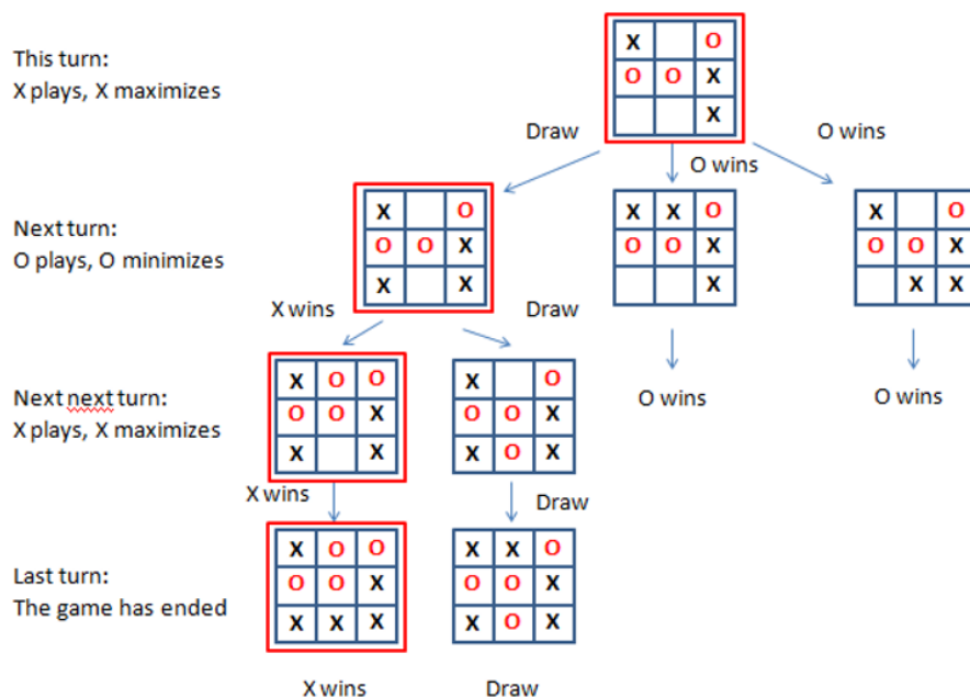
FIGURE 3-3: A glance at min-max approximation in a tic-tac-toe game.
